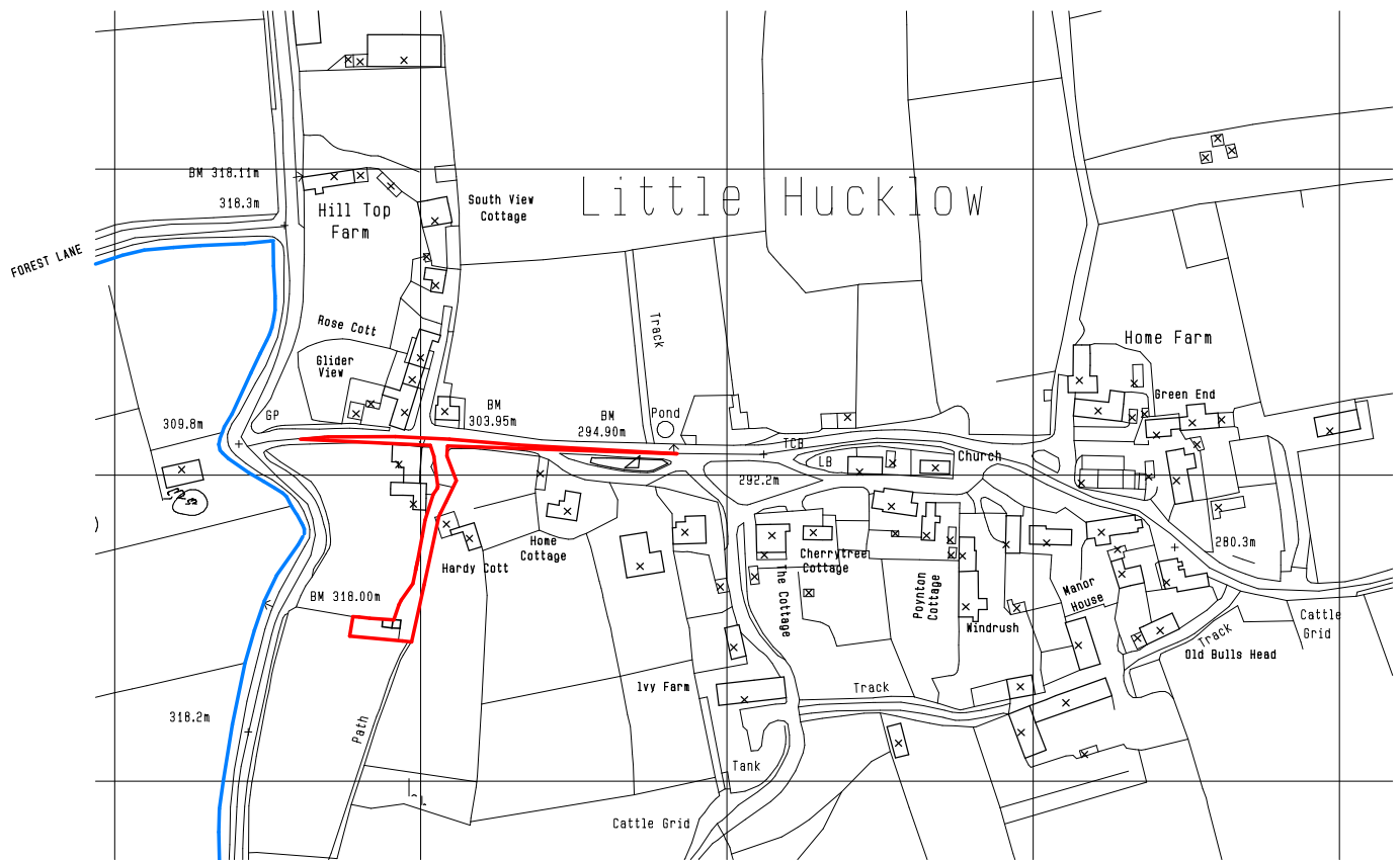
SITE LOCATION PLAN SCALE 1:2500 RETROSPECTIVE APPLICATION FOR CONVERSION OF BARN TO LOCAL NEED AFFORDABLE DWELLING AT 'THE FOLD', LITTLE HUCKLOW FOR MISS A BRADBURY
